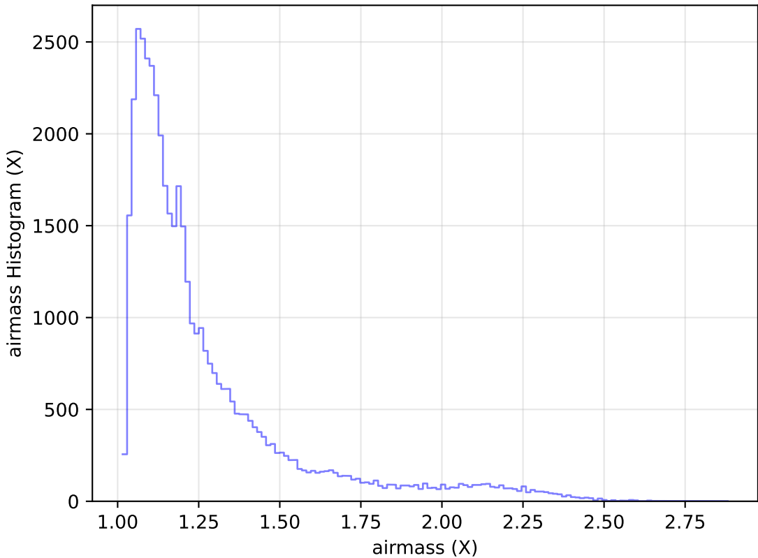
weather_cloudso31v3.4_10yrs Yr 1 r band: airmass Histogram
