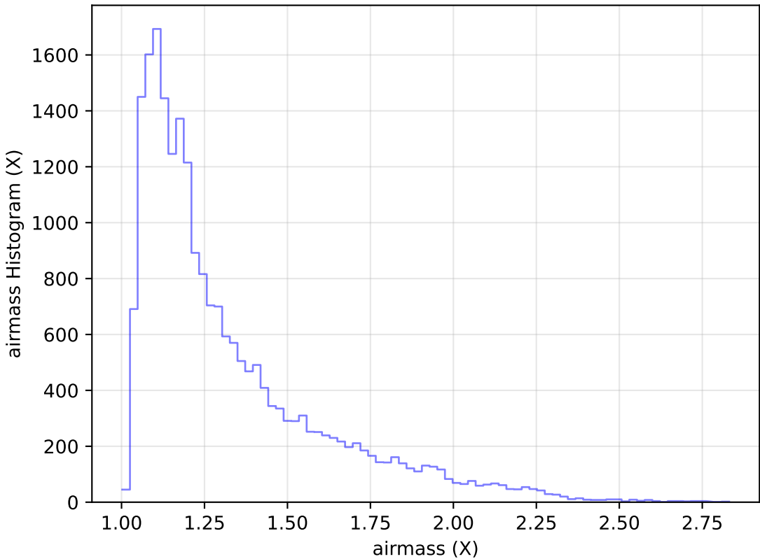
weather_cloudso31v3.4_10yrs Yr 1 g band: airmass Histogram
