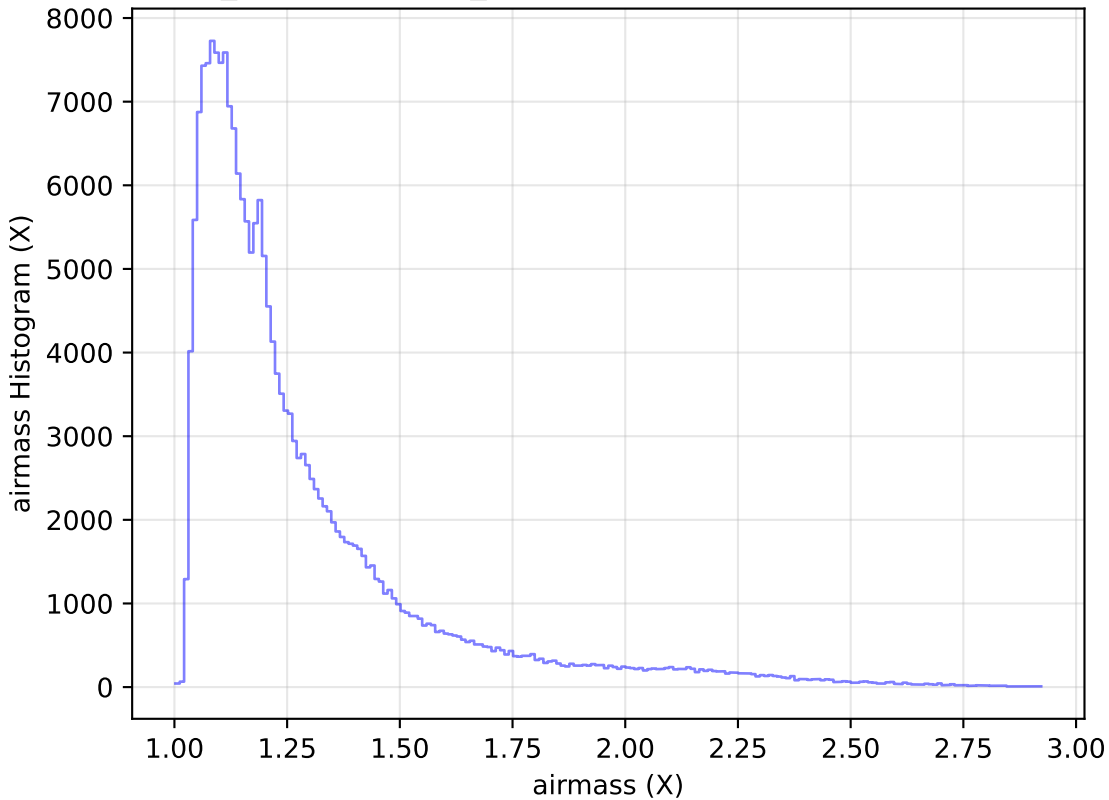
weather_cloudso31v3.4_10yrs Yr 1 all bands: airmass Histogram
