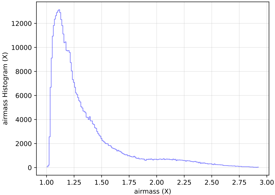
weather_cloudso31v3.4_10yrs WFD z band: airmass Histogram
