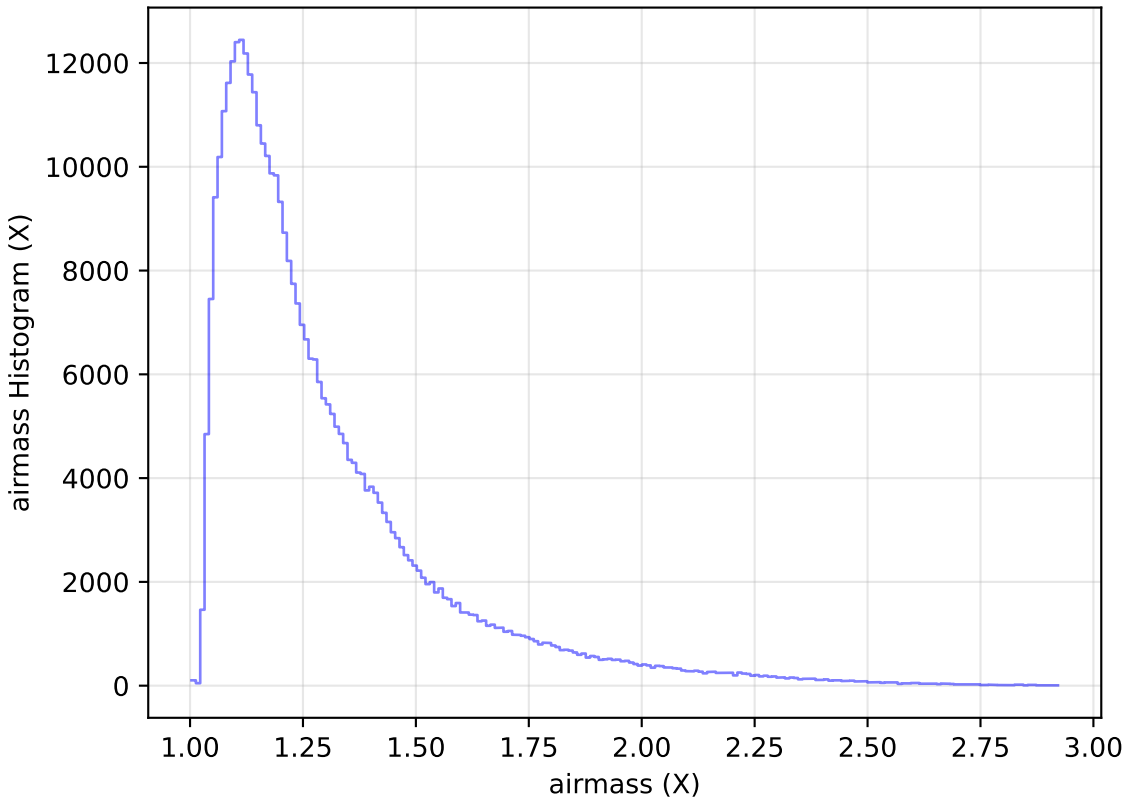
weather_cloudso31v3.4_10yrs WFD y band: airmass Histogram
