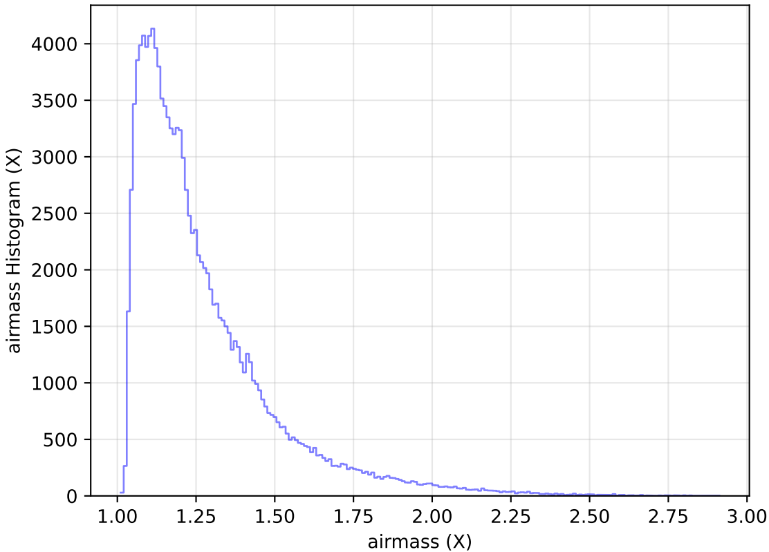
weather_cloudso31v3.4_10yrs WFD u band: airmass Histogram
