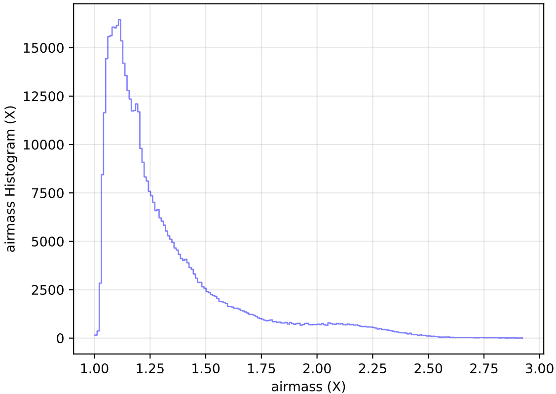
weather_cloudso31v3.4_10yrs WFD r band: airmass Histogram
