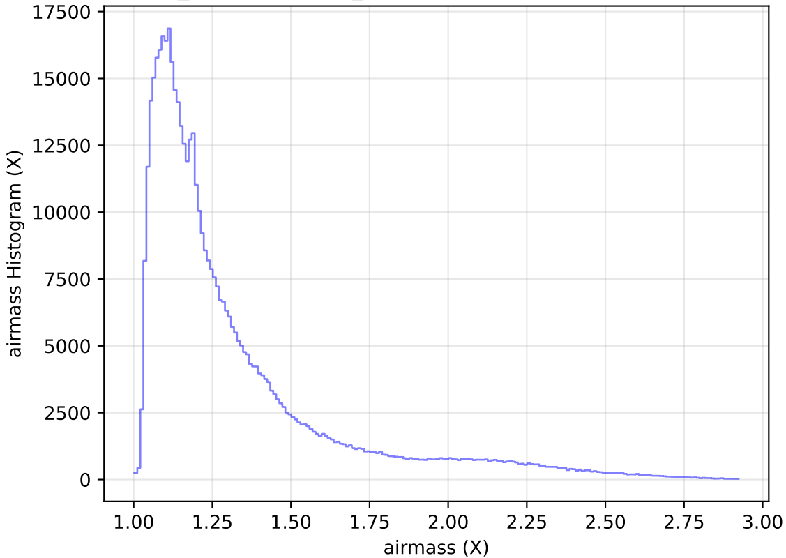
weather_cloudso31v3.4_10yrs WFD i band: airmass Histogram
