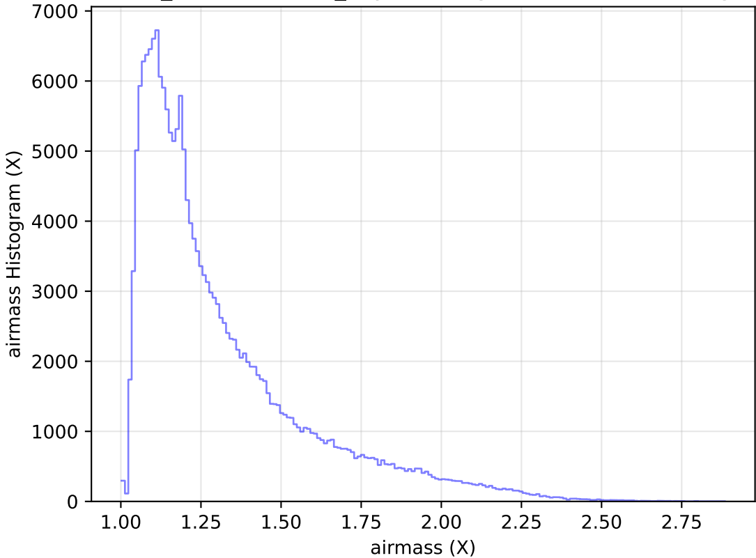
weather_cloudso31v3.4_10yrs WFD g band: airmass Histogram
