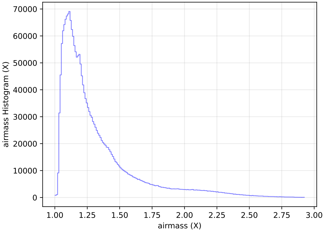
weather_cloudso31v3.4_10yrs WFD all bands: airmass Histogram
