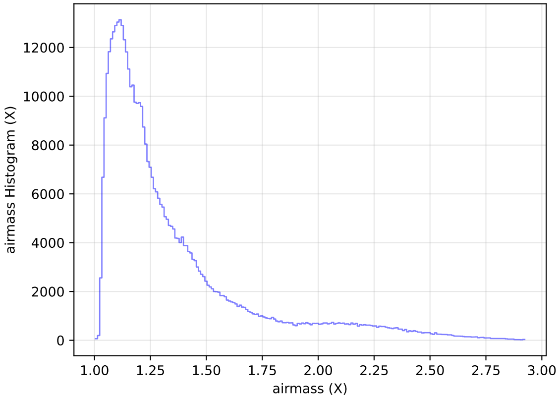
weather_cloudso31v3.4_10yrs All sky z band: airmass Histogram
