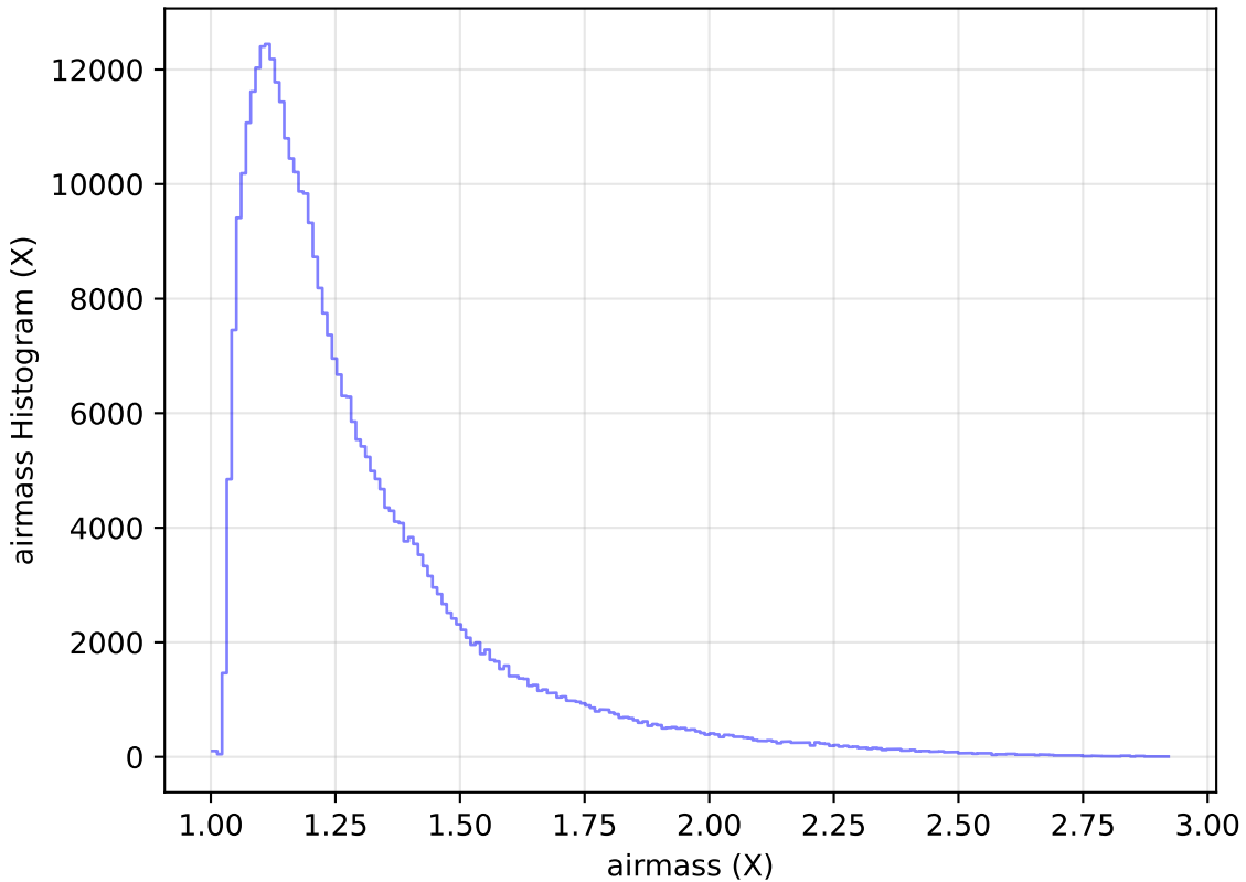
weather_cloudso31v3.4_10yrs All sky y band: airmass Histogram
