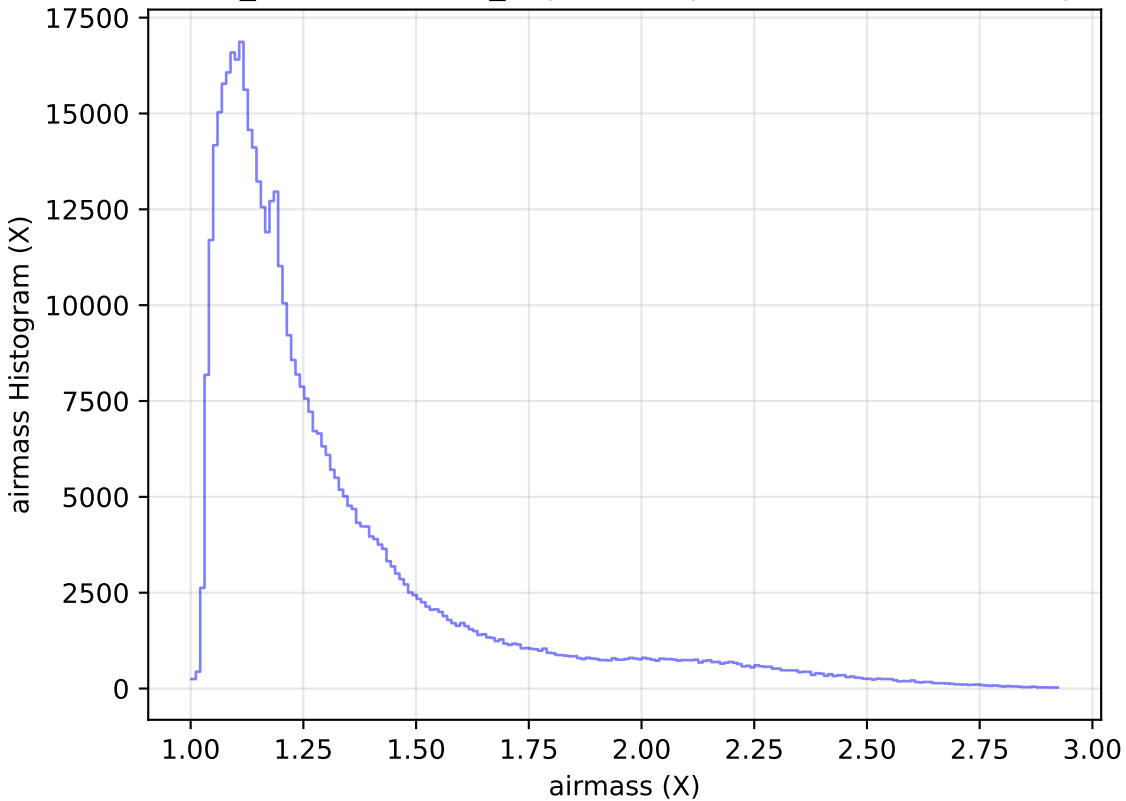
weather_cloudso31v3.4_10yrs All sky i band: airmass Histogram
