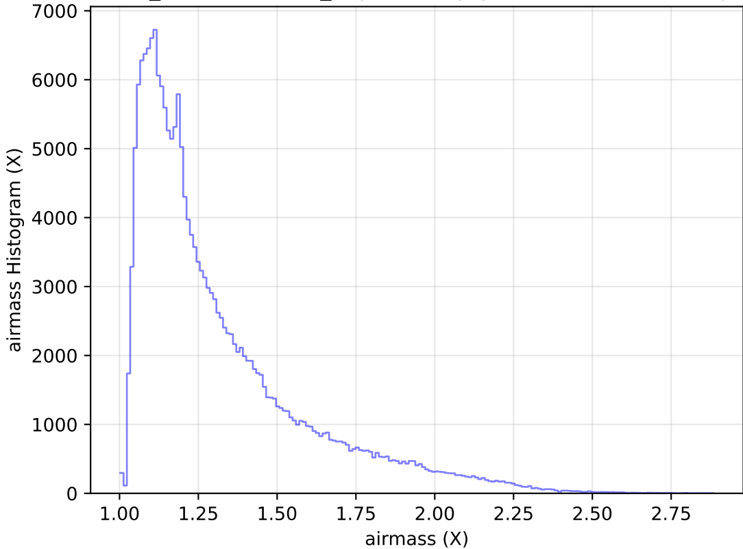
weather_cloudso31v3.4_10yrs All sky g band: airmass Histogram
