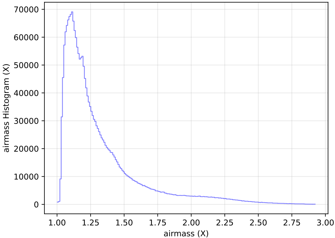
weather_cloudso31v3.4_10yrs All sky all bands: airmass Histogram
