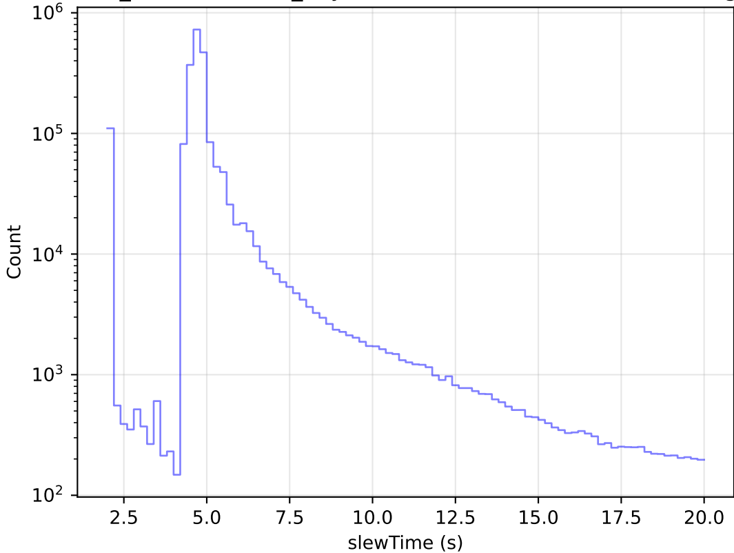
weather_cloudso31v3.4_10yrs All visits: Zoom Slew Time Histogram
