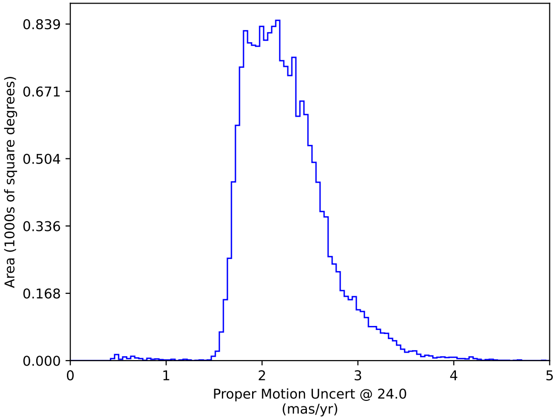
weather_cloudso31v3.4_10yrs WFD: Proper Motion Uncert @ 24.0
