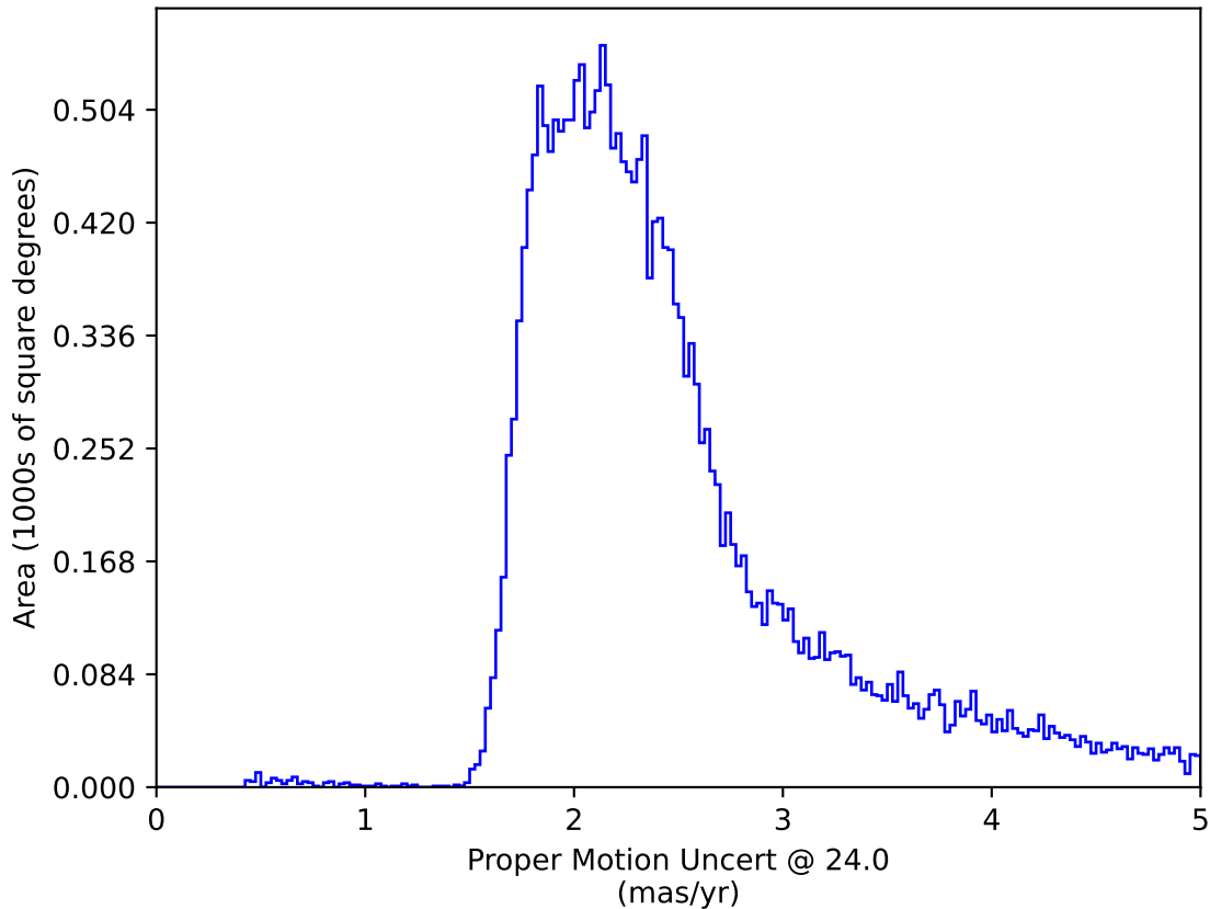
weather_cloudso31v3.4_10yrs All sky: Proper Motion Uncert @ 24.0
