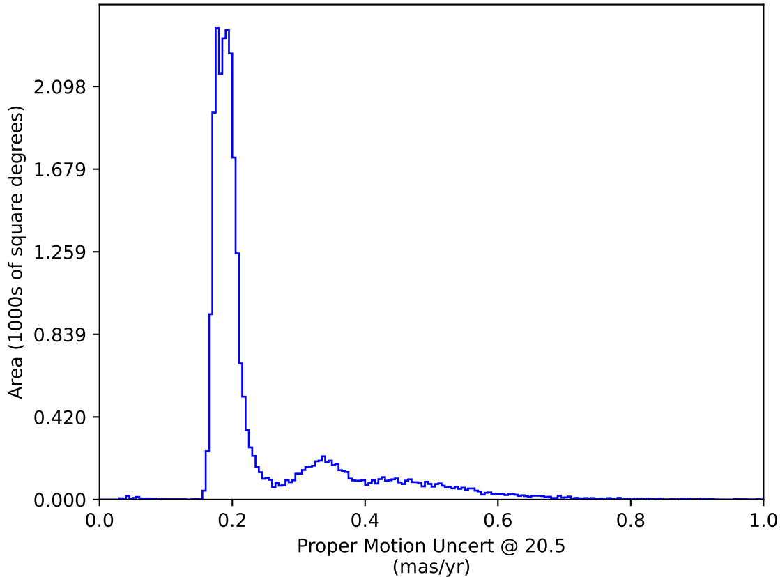
weather_cloudso31v3.4_10yrs All sky: Proper Motion Uncert @ 20.5
