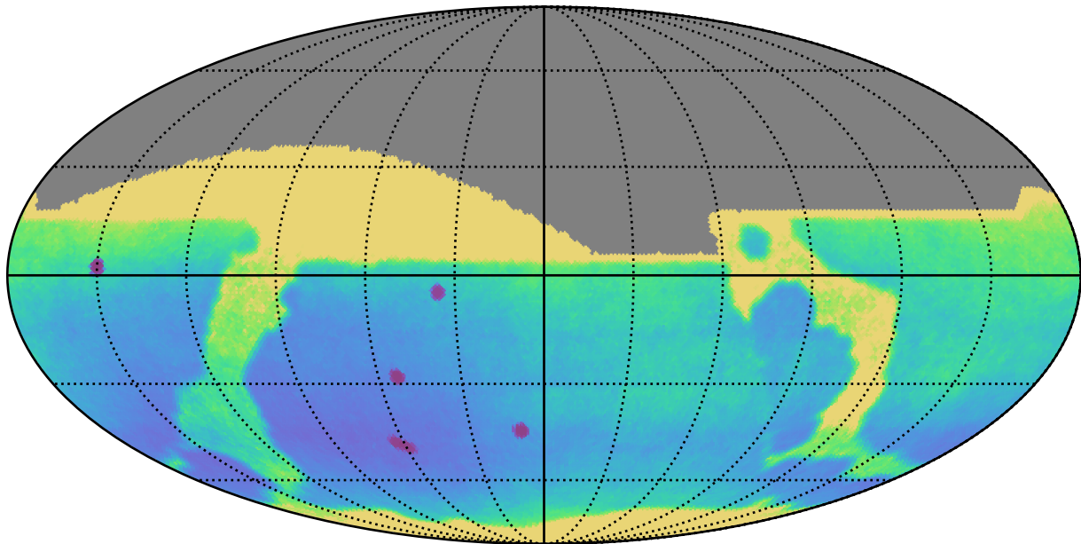
weather_cloudso31v3.4_10yrs All sky: Parallax Uncert @ 24.0
