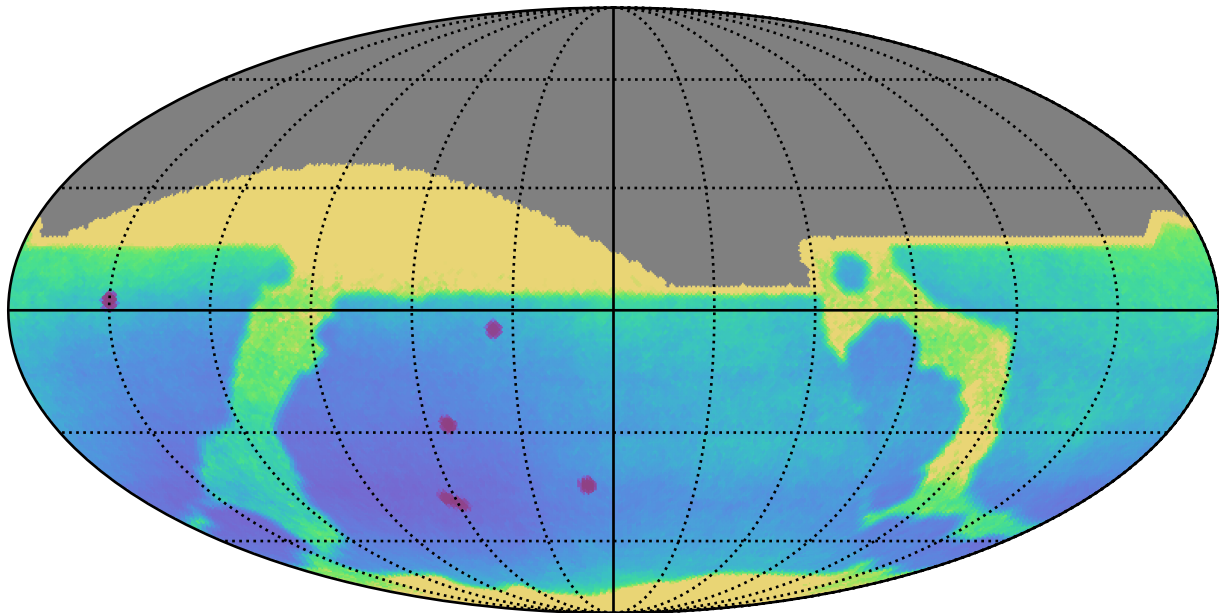
weather_cloudso31v3.4_10yrs All sky: Parallax Uncert @ 22.4
