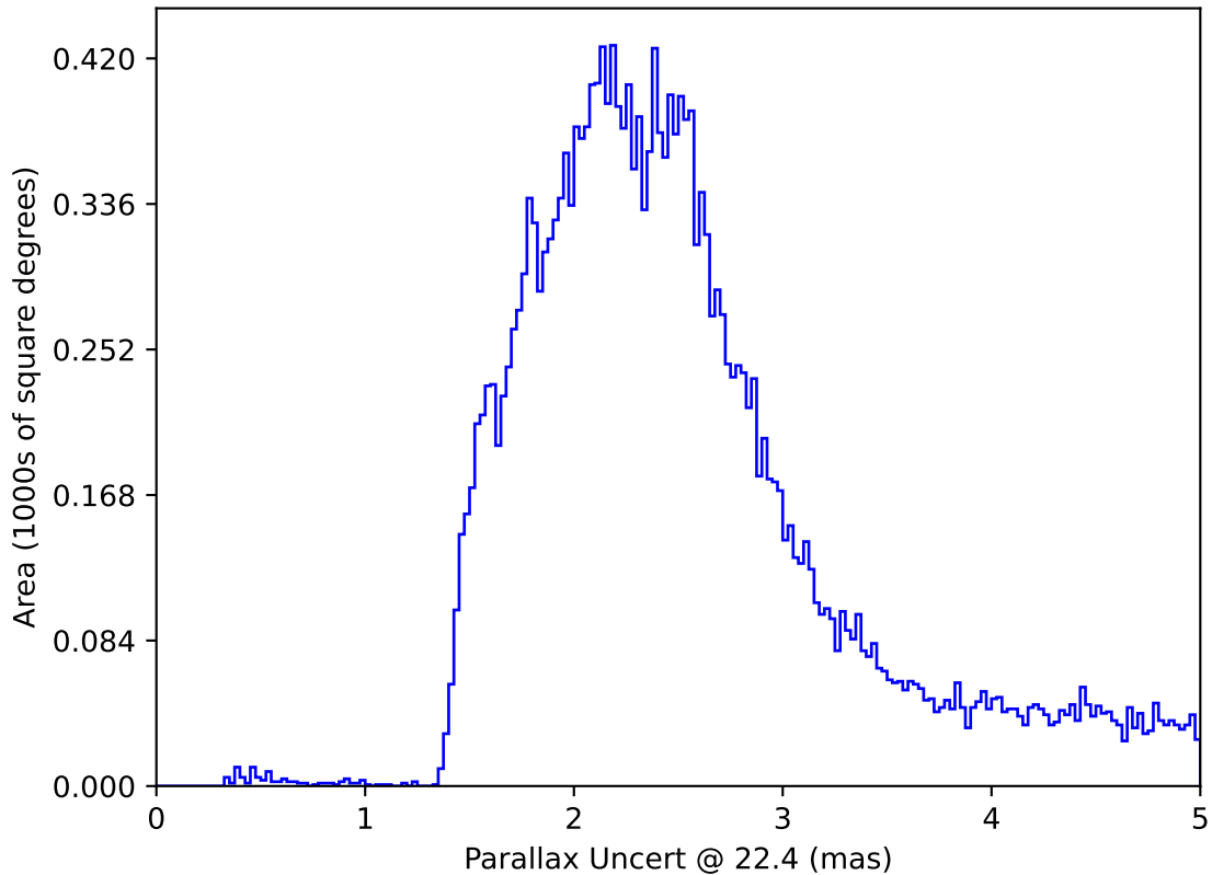
weather_cloudso31v3.4_10yrs All sky: Parallax Uncert @ 22.4
