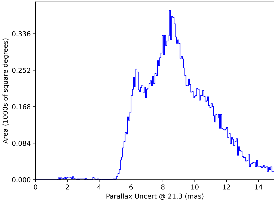
weather_cloudso31v3.4_10yrs All sky y band only: Parallax Uncert @ 21.3
