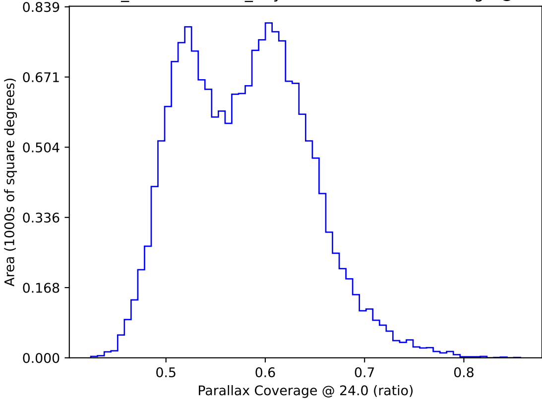
weather_cloudso31v3.4_10yrs WFD: Parallax Coverage @ 24.0
