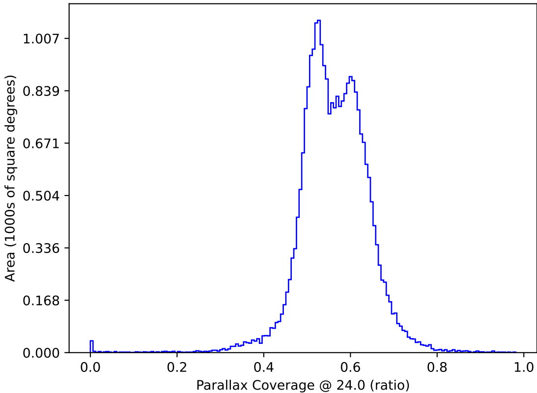
weather_cloudso31v3.4_10yrs All sky: Parallax Coverage @ 24.0
