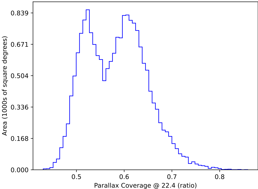
weather_cloudso31v3.4_10yrs WFD: Parallax Coverage @ 22.4
