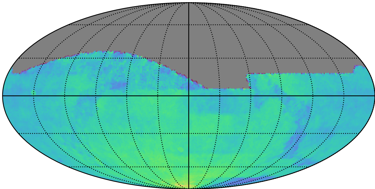
weather_cloudso31v3.4_10yrs All sky: Parallax Coverage @ 22.4
