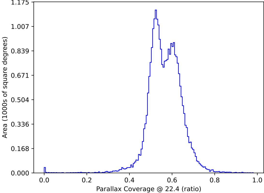
weather_cloudso31v3.4_10yrs All sky: Parallax Coverage @ 22.4
