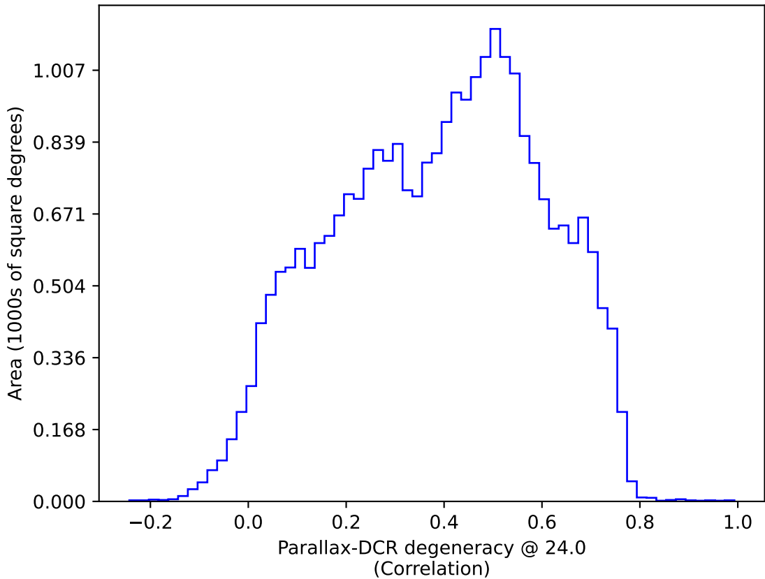
weather_cloudso31v3.4_10yrs All sky: Parallax-DCR degeneracy @ 24.0
