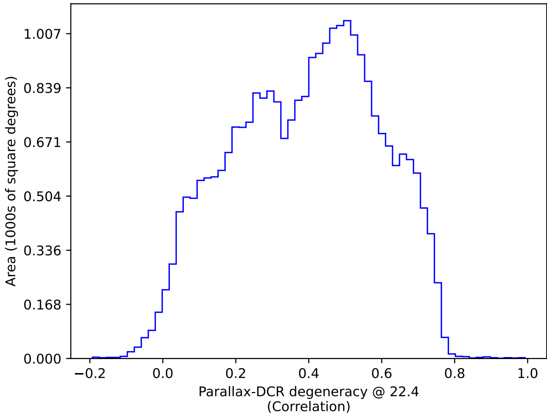
weather_cloudso31v3.4_10yrs All sky: Parallax-DCR degeneracy @ 22.4
