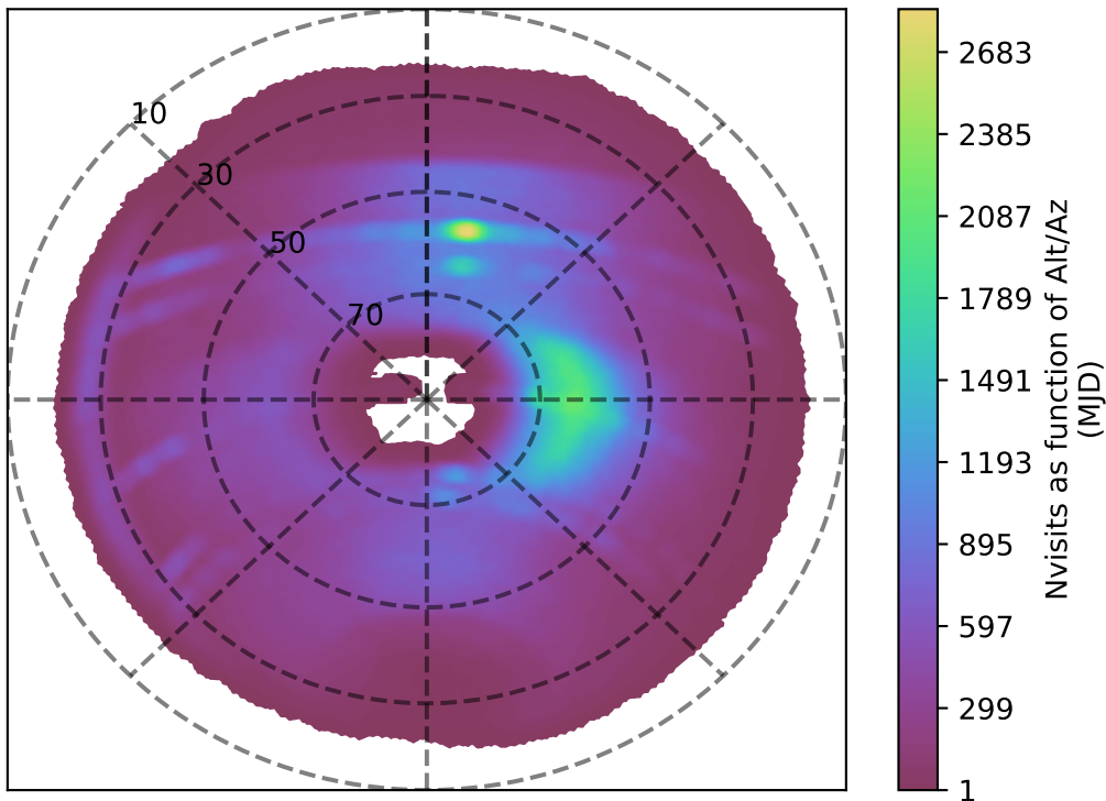
weather_cloudso31v3.4_10yrs r band: Nvisits as function of Alt/Az
