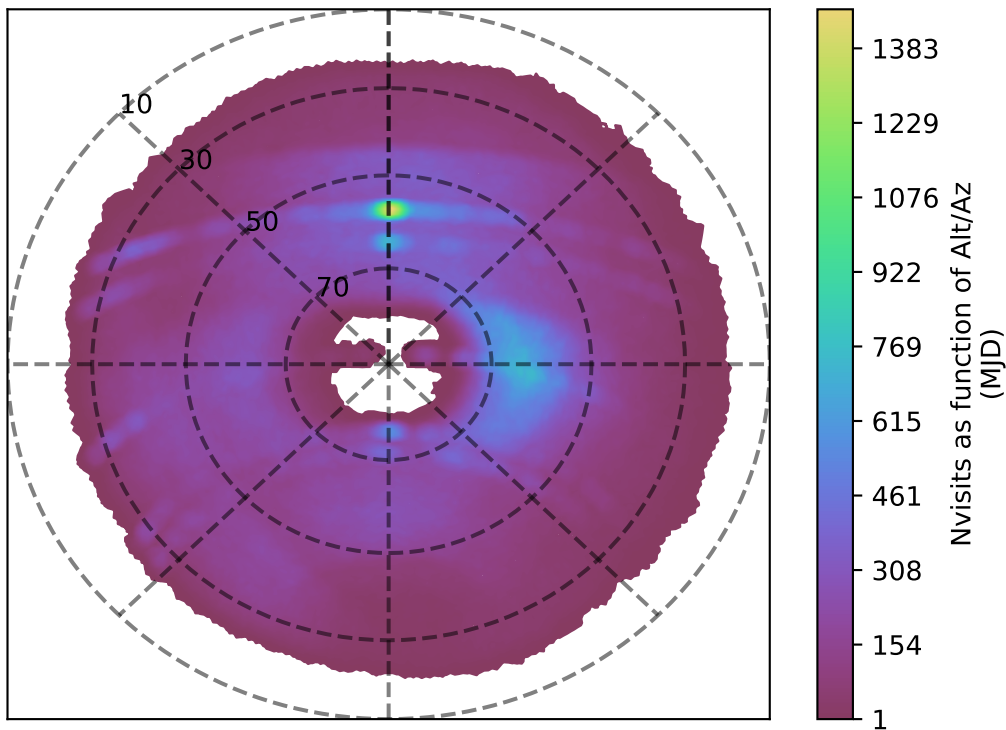
weather_cloudso31v3.4_10yrs g band: Nvisits as function of Alt/Az
