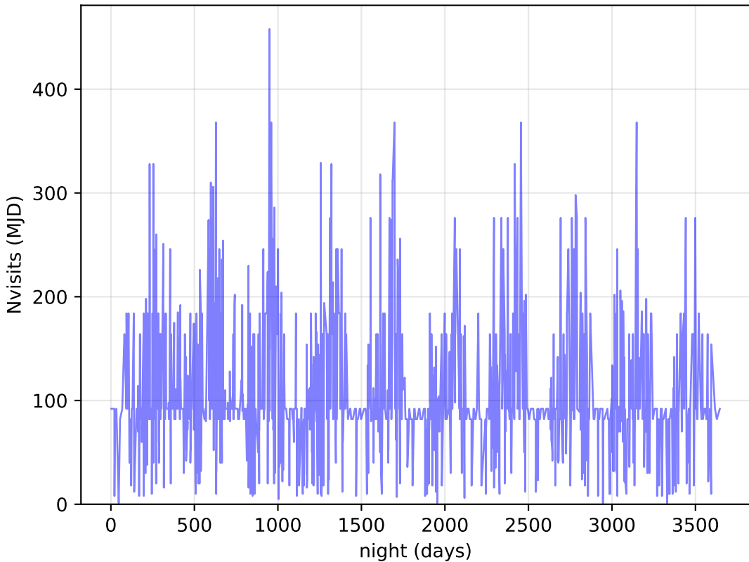
weather_cloudso31v3.4_10yrs DDF: Nvisits
