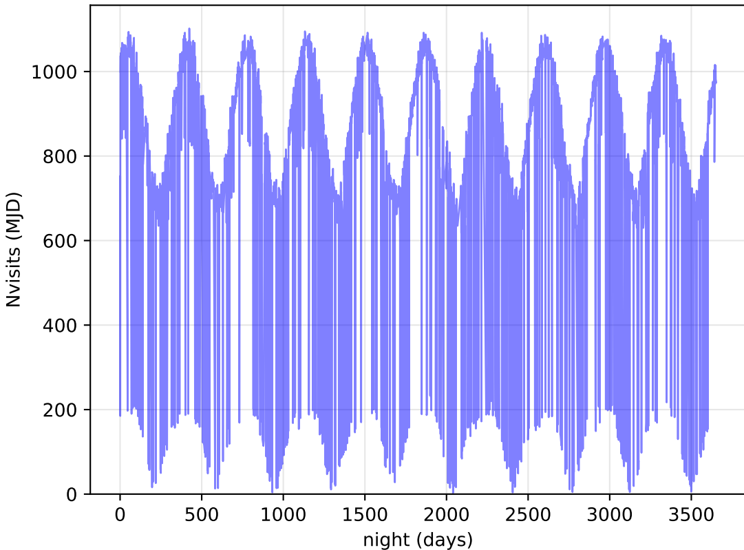
weather_cloudso31v3.4_10yrs All visits: Nvisits
