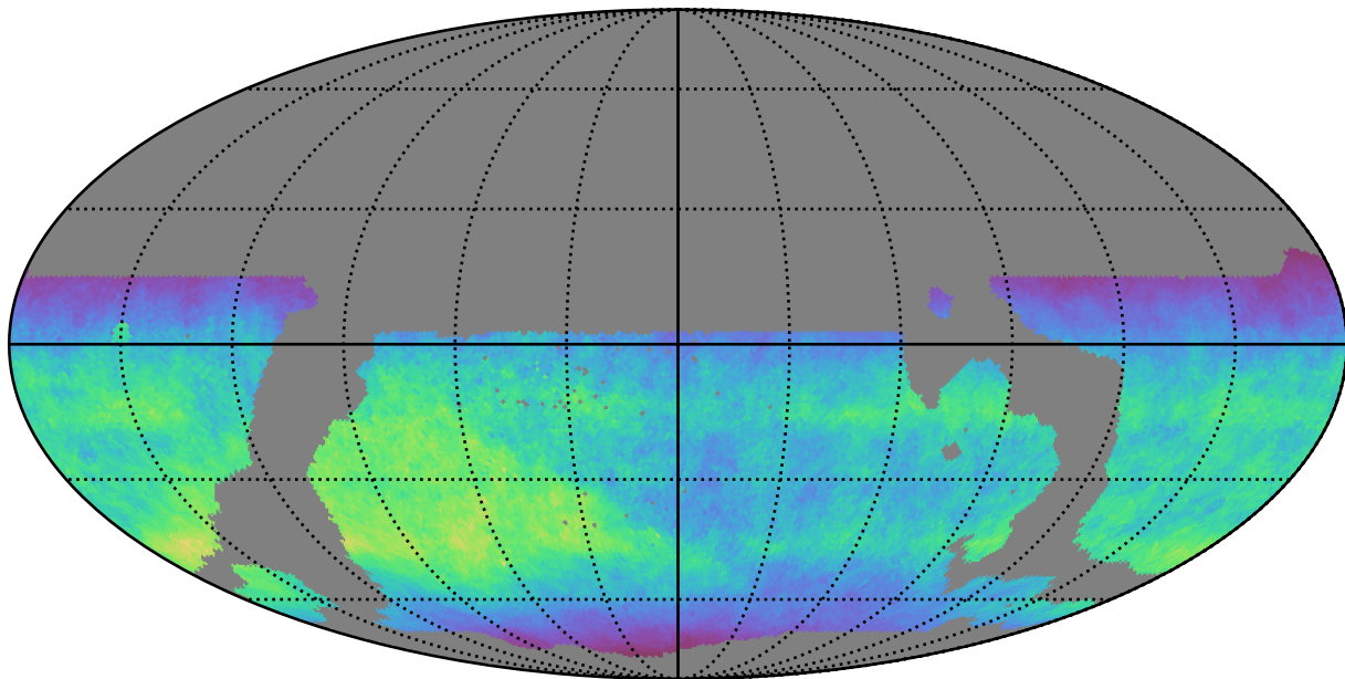
weather_cloudso31v3.4_10yrs WFD z band: Normalized Teff
