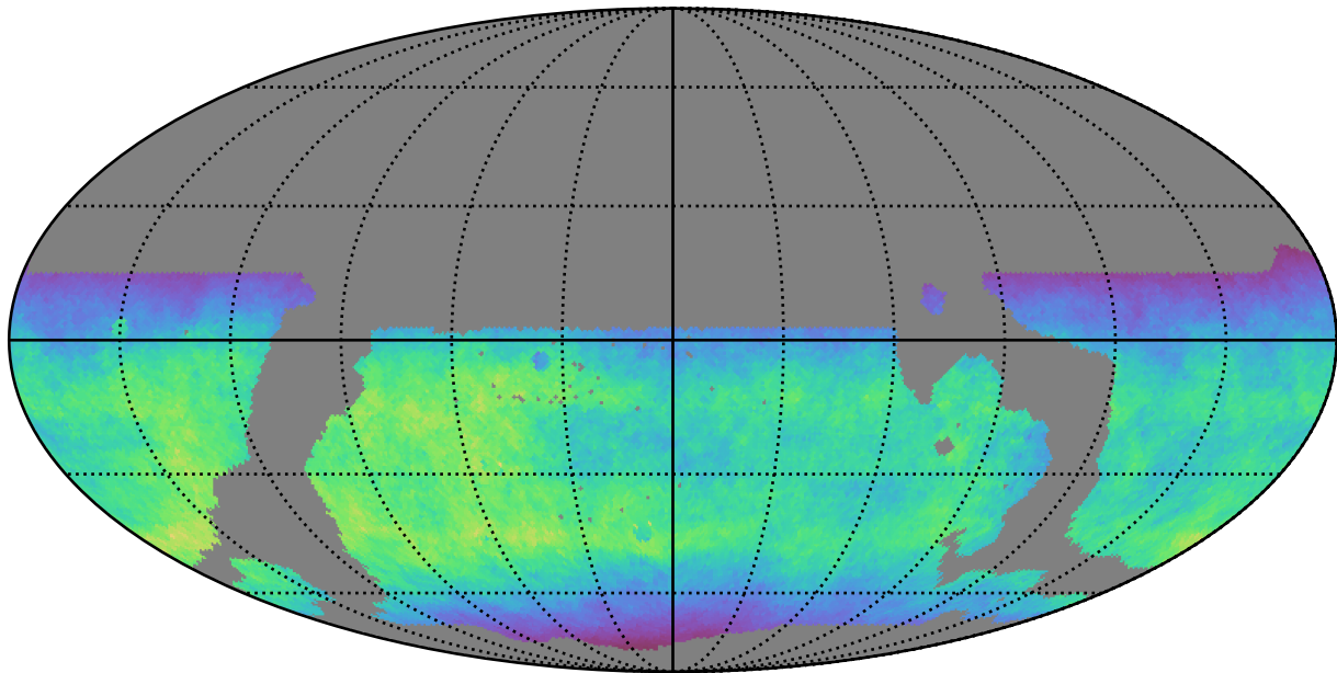
weather_cloudso31v3.4_10yrs WFD y band: Normalized Teff
