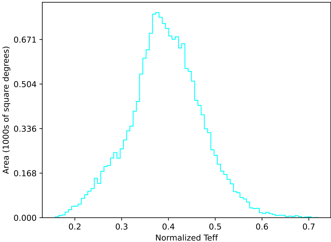
weather_cloudso31v3.4_10yrs WFD u band: Normalized Teff
