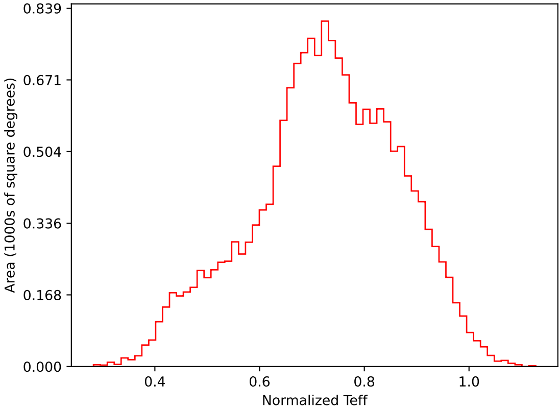
weather_cloudso31v3.4_10yrs WFD i band: Normalized Teff
