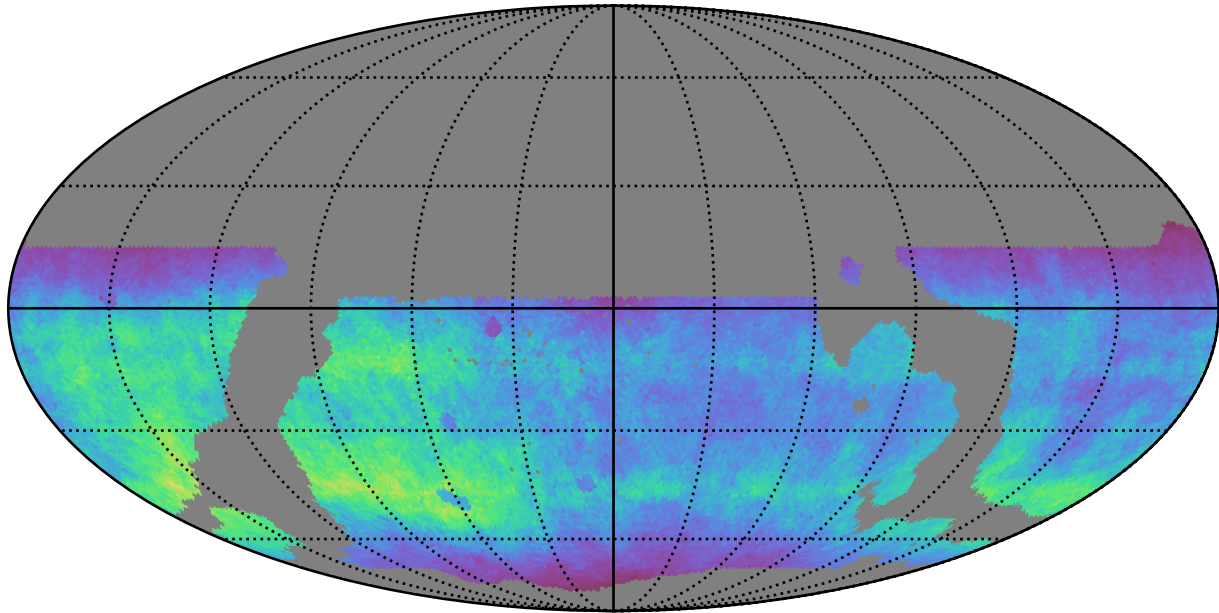
weather_cloudso31v3.4_10yrs WFD g band: Normalized Teff
