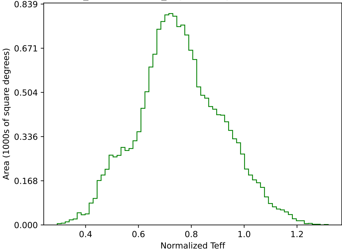
weather_cloudso31v3.4_10yrs WFD g band: Normalized Teff
