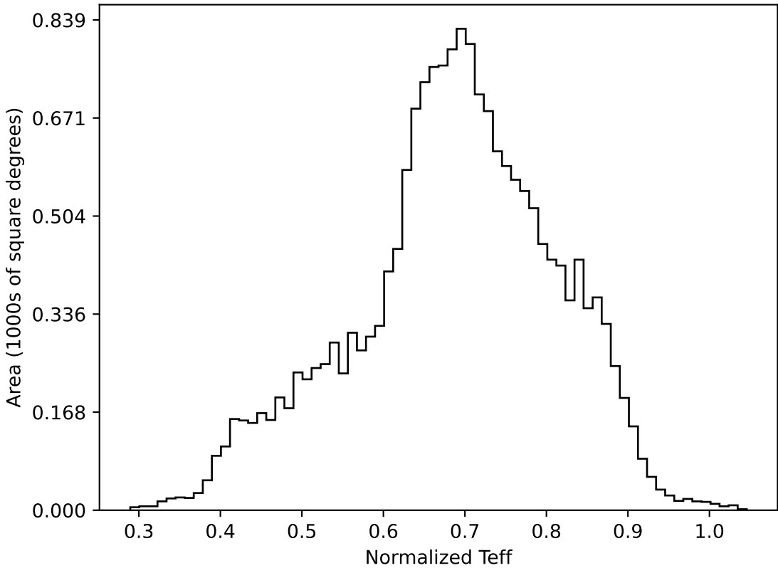
weather_cloudso31v3.4_10yrs WFD all bands: Normalized Teff
