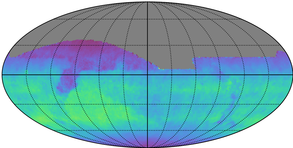
weather_cloudso31v3.4_10yrs All sky z band: Normalized Teff
