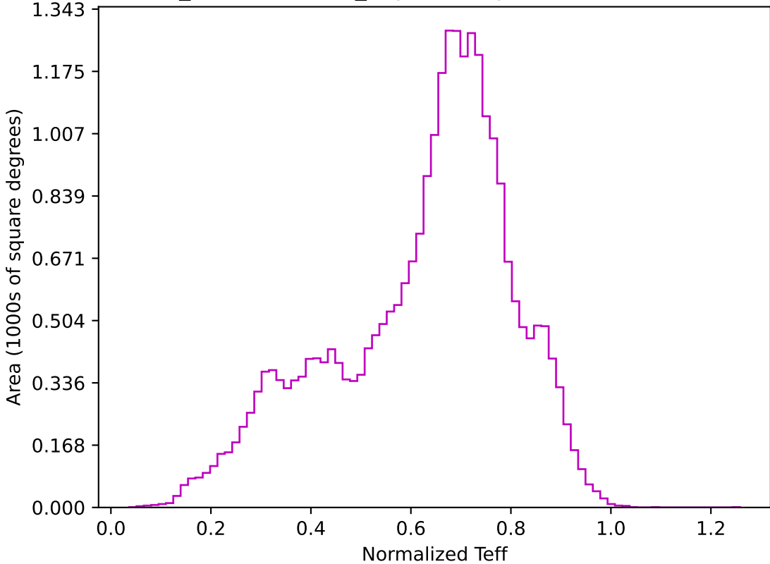
weather_cloudso31v3.4_10yrs All sky z band: Normalized Teff
