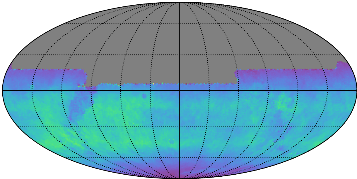
weather_cloudso31v3.4_10yrs All sky y band: Normalized Teff
