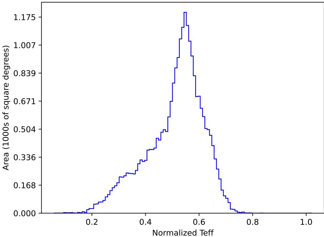
weather_cloudso31v3.4_10yrs All sky y band: Normalized Teff
