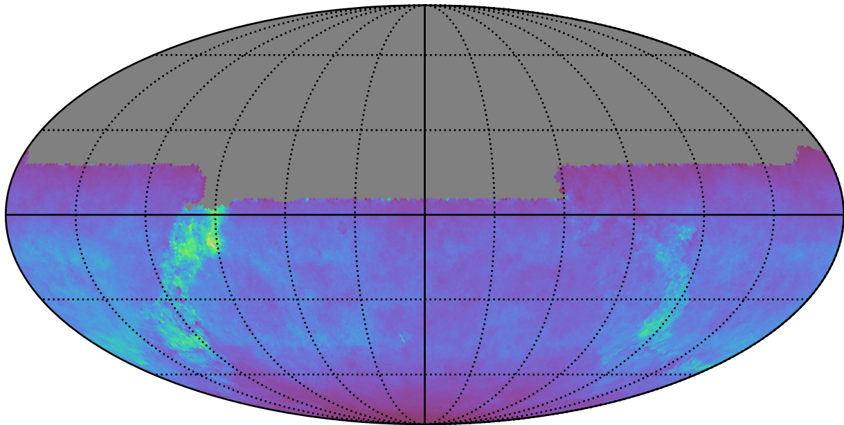
weather_cloudso31v3.4_10yrs All sky u band: Normalized Teff
