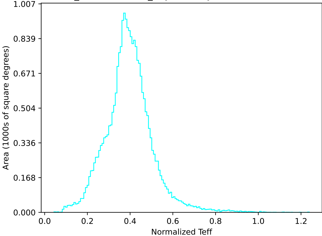
weather_cloudso31v3.4_10yrs All sky u band: Normalized Teff
