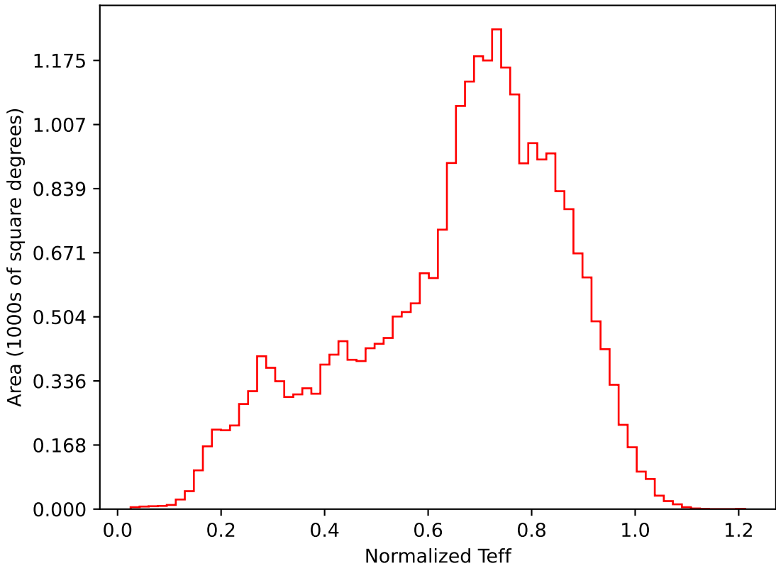
weather_cloudso31v3.4_10yrs All sky i band: Normalized Teff
