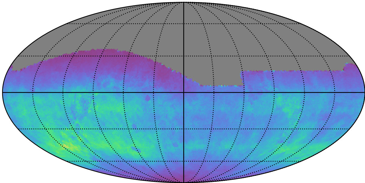
weather_cloudso31v3.4_10yrs All sky g band: Normalized Teff
