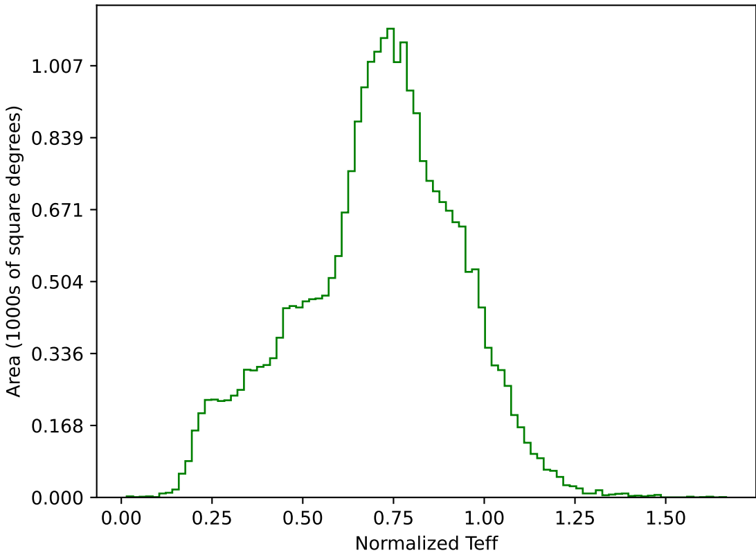
weather_cloudso31v3.4_10yrs All sky g band: Normalized Teff
